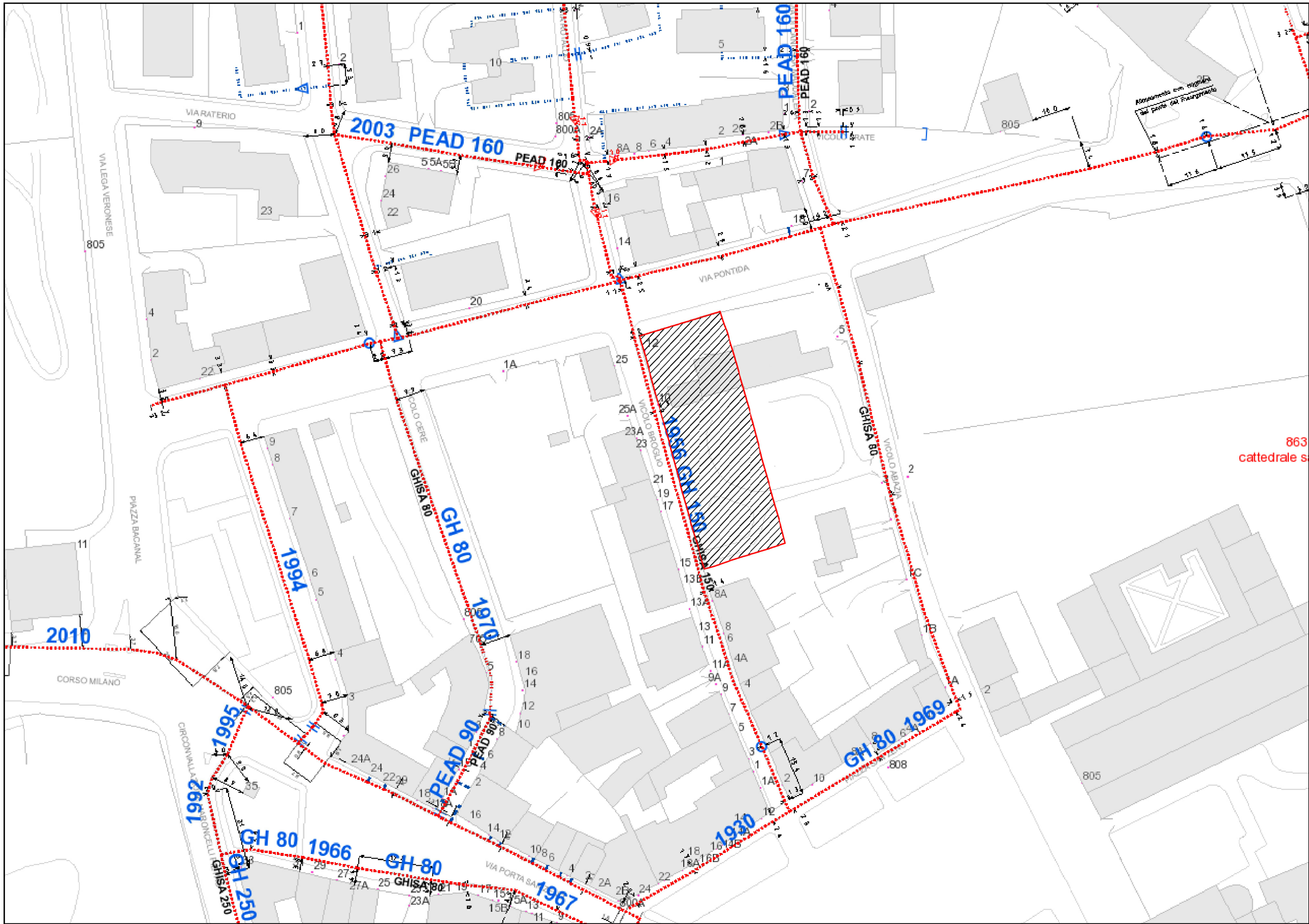
Schema rete gas
